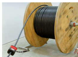
RM35 with RUNPOLIFTER L1600 and 3 x 35 mm 2 cable
